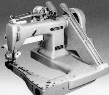
▲FA-S BROTHER DT6-B925 Feed-off-Arm Chain stitch, Solenoid Type (솔자동)
