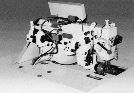
▲ST-A SUNSTAR KM-235 Single Needle Lockstitch, Air Type (에어식)
